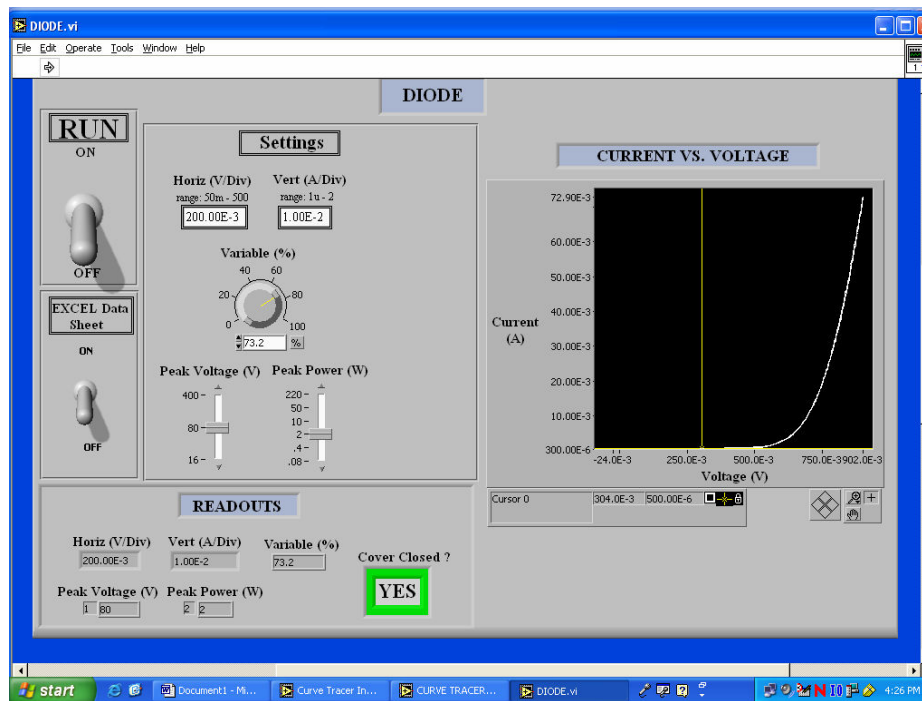
Figure 3: Typical LabVIEW interface panel for Tektronix 370: diode
