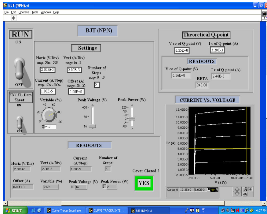
Figure 4: Typical LabVIEW interface panel for Tektronix 370: BJT (NPN)
