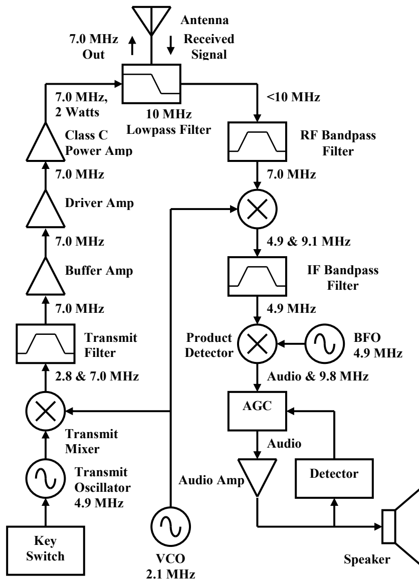
Fig. 1. Block diagram of the NorCal 40A transceiver.
