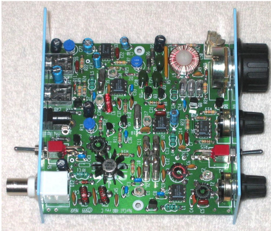
Fig. 2. Photograph of assembled transceiver.
