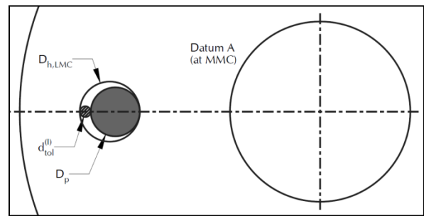
Fig. 4, Diagram used to determine position tolerance for case (I).
