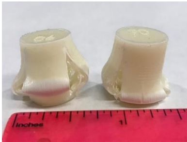
Figure 23. ABS Specimens of Sparse Structure Printed by Fortus at flat-90° Print Orientation After Compression Test.
