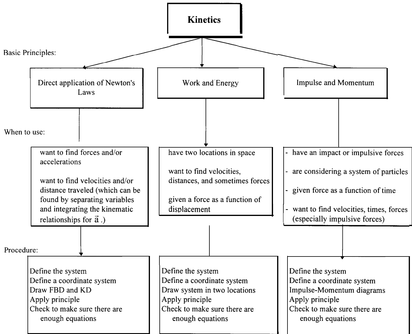
Figure 6- Concept map for kinetics designed to help students identify the principles to apply when solving problems.
