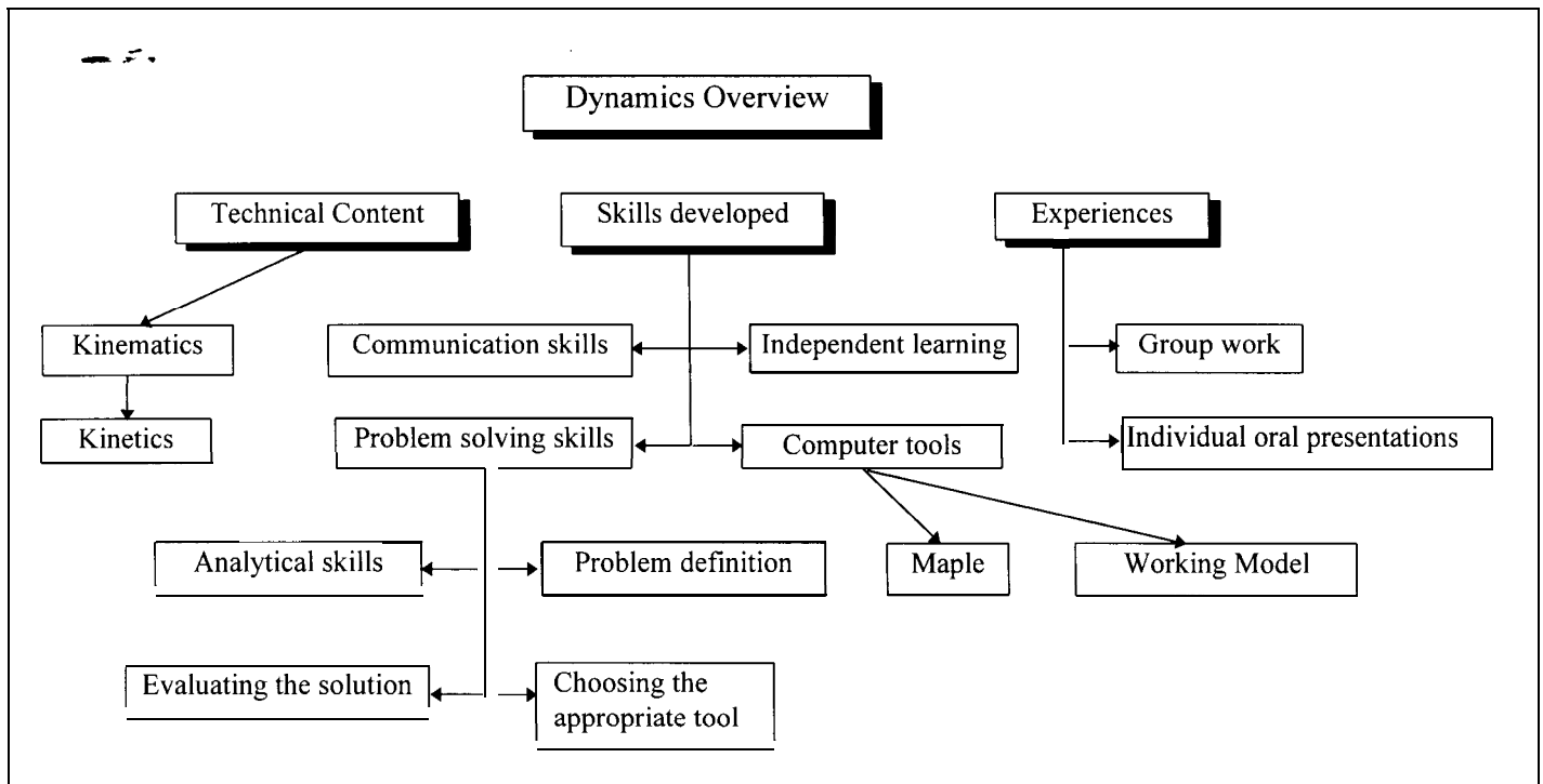
Figure 4- Overview of the goals for a dynamics course.
