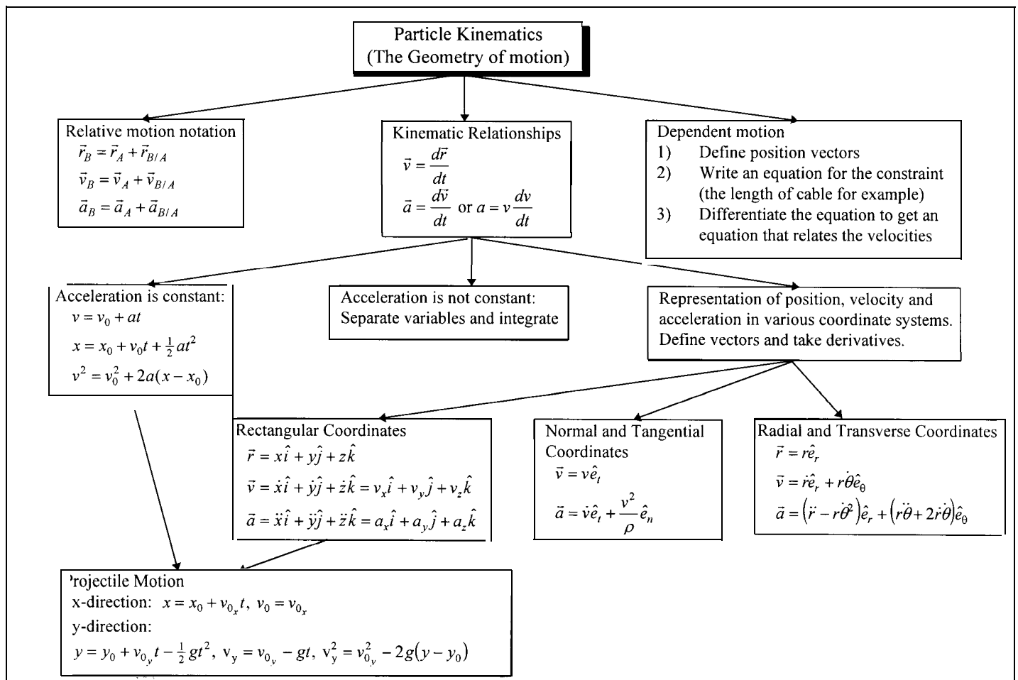
Figure 5 - Concept map for the topics in particle kinematics.
