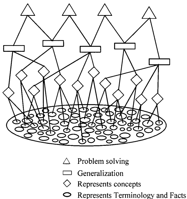
Figure 1- Phases in a learning hierarchal.
