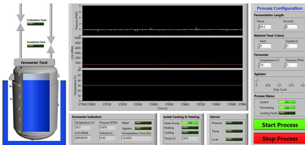
Figure 6: Bioreactor-1 Human Machine Interface (HMI)
