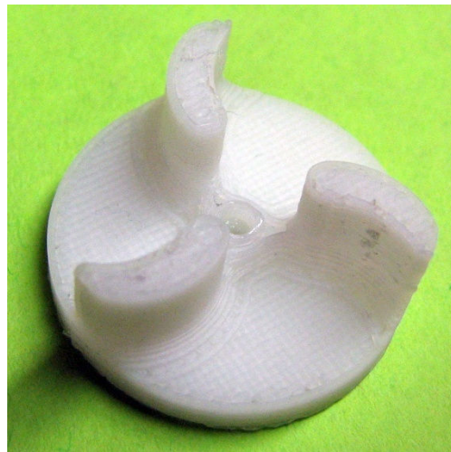
Figure 3 – Rapid Prototyped Impeller
