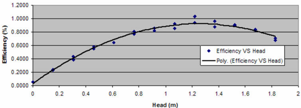
Figure 15 – Student Generated Plot of Pump Efficiency Versus Head
