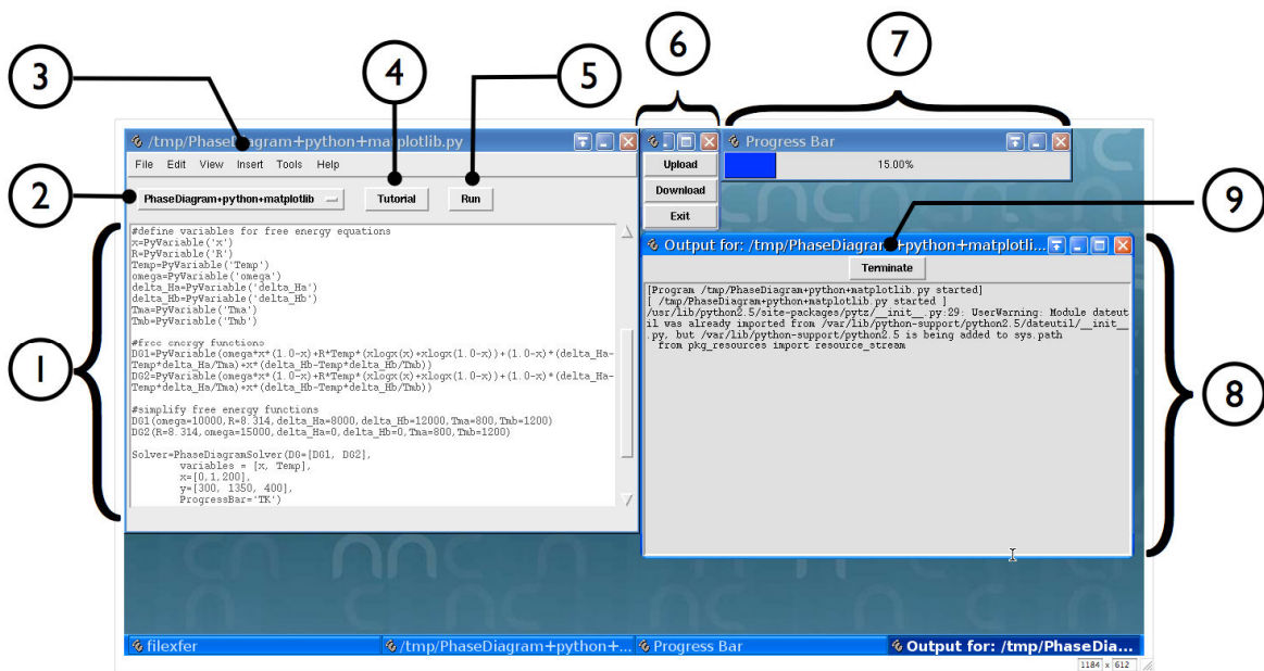
Figure 2. VKML-Live web-based interface. Python scripts are edited online at 1, while the user can select from a variety of examples at 2. The toolbar is shown at 3, where the user can perform standard editing operations, such as copy and paste. For a selected script, a link to any available tutorial can be deployed by clicking at 4. Edited or default scripts can be run at 5. Data, modified programs, images, and databases can be exchanged through the interface provided at 6. Regardless of the deployed application instantiating or not a GUI such as the one shown at 7, a process control window will be deployed, 8, which can be terminated by clicking at 9.
