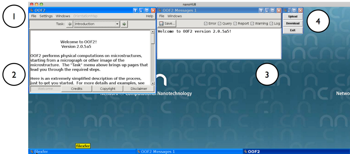
Figure 1. OOF2 web-based interface. At 1, finite element meshes and material properties are uploaded, while at 2, the user selects among an array of menu items operations to perform on the material microstructures. At 3, executed commands, errors and the status of the system are reported. Through the Filexfer, files are uploaded and downloaded: microstructures are added to the system, while macroscopic material properties are reported.
