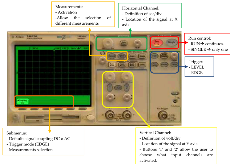
Figure 4: Main functionalities of the digital oscilloscope
