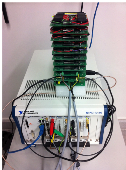
Figure 1: VISIR remote lab set up at University of Deusto, Spain
