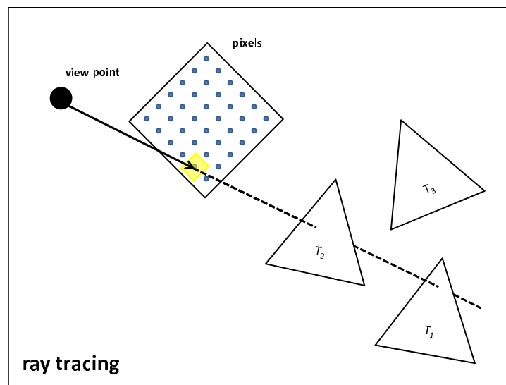
Figure 3: The ray tracing algorithm. Rays (3D half-lines) originating at the view point are traced into the scene, and the object closest to the view point is found. Here, the 3D line query determines that triangle T_2 is visible through the highlighted pixel.
