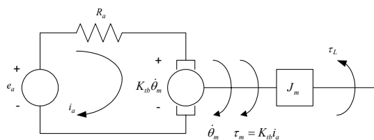
Figure 7: DC Motor Representation
