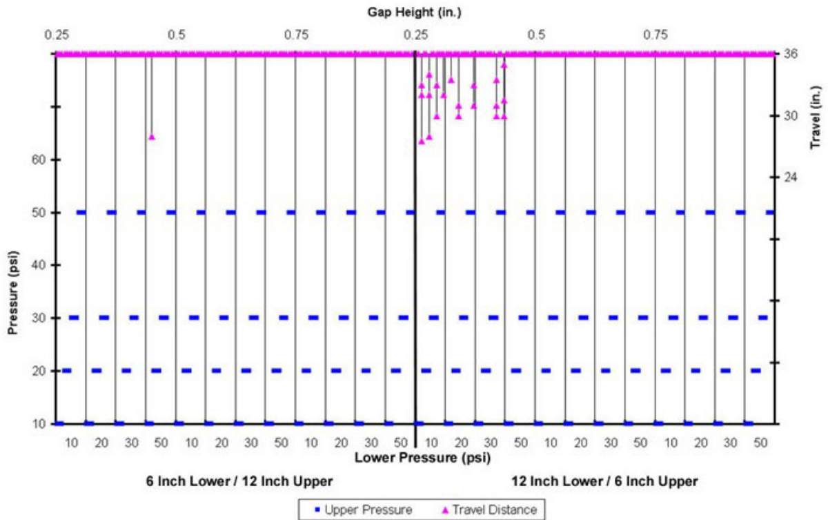
Figure 3. Multi-dimensional plot of experimental data from a design experiment
